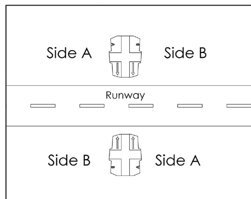
Figure 1: Light Placement
