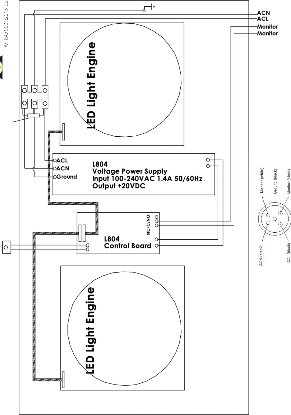
RGL Removeable Plug Details
