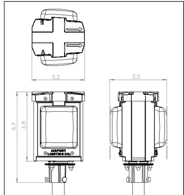
Fixture Dimensions
