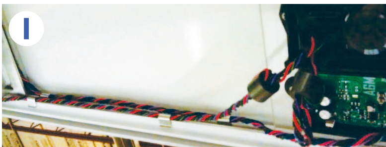
C7-LVCV2 power supply and C7-DRVR driver with wire harnesses secured by u-clips.
