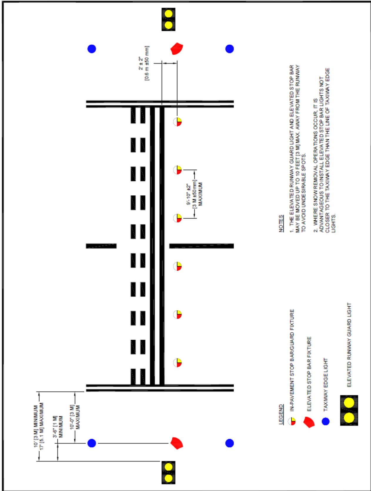
Figure 1: FAA Guard Light Field Placement (from AC 150/5340-30)
