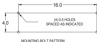
MOUNTING BOLT PATTERN
